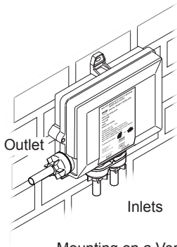
Mounting on a Vertical Surface
